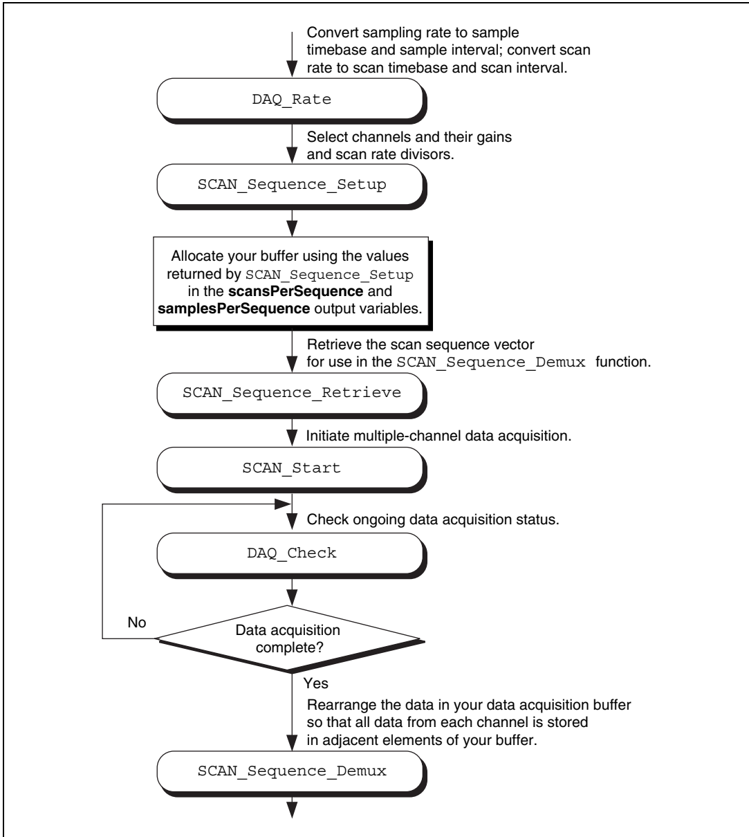
Figure 3-11. Multirate Scanning
